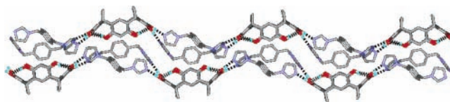
Figure 1. Double-buckled chainlike polymer formed by CMCR and bix.
